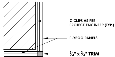
OUTSIDE CORNER PLAN DETAIL
