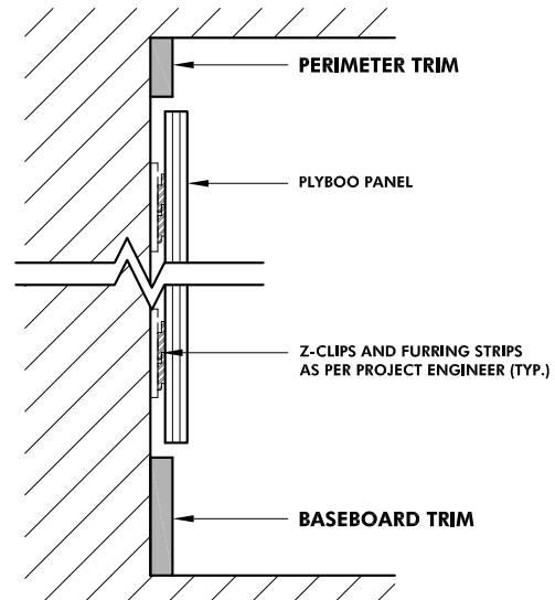
PERIMETER TRIM / BASEBOARD SECTION DETAILS
